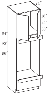
Micro/Oven Cabinet 2 Doors, 2 Drawers
